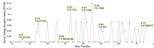
Fig. 3. NVSI Makassar distribution system, feeder Kima, 76 buses
